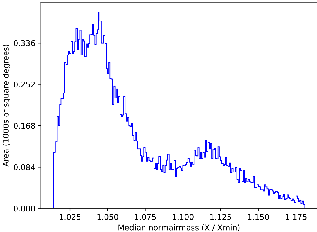
scp_reweight_v3.3_10yrs All sky r band: Median normairmass
