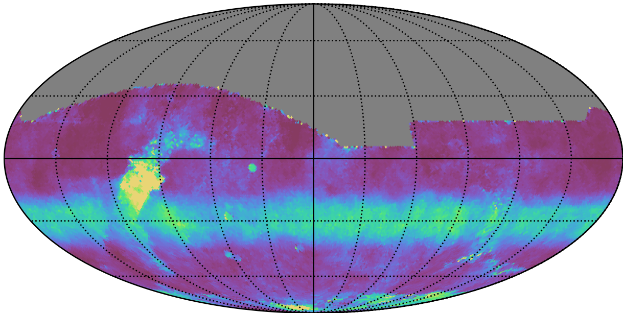
scp_reweight_v3.3_10yrs All sky i band: Median normairmass
