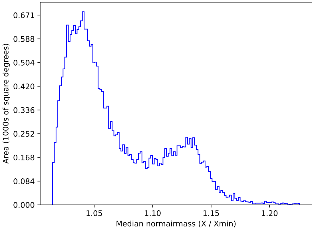
scp_reweight_v3.3_10yrs All sky i band: Median normairmass
