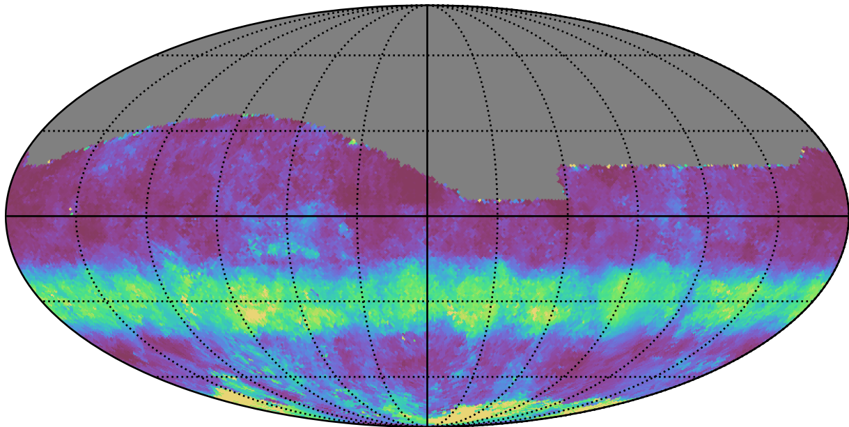
scp_reweight_v3.3_10yrs All sky g band: Median normairmass
