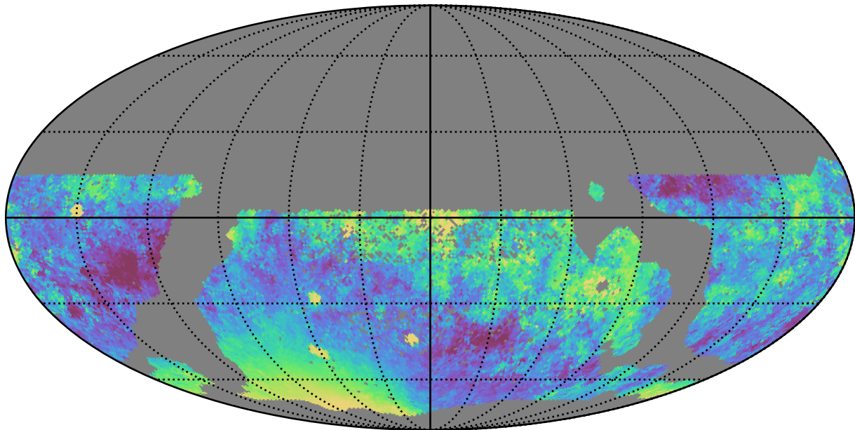
scp_reweight_v3.3_10yrs WFD z band: Median moonDistance
