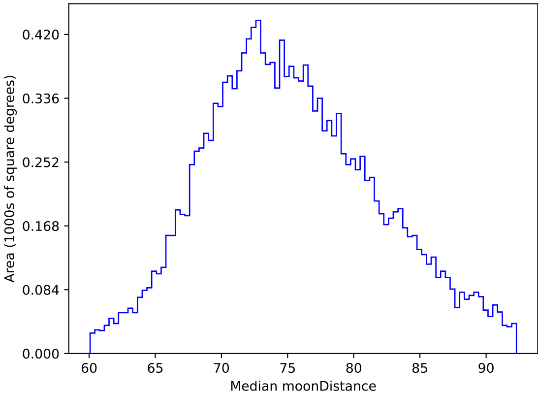
scp_reweight_v3.3_10yrs WFD z band: Median moonDistance
