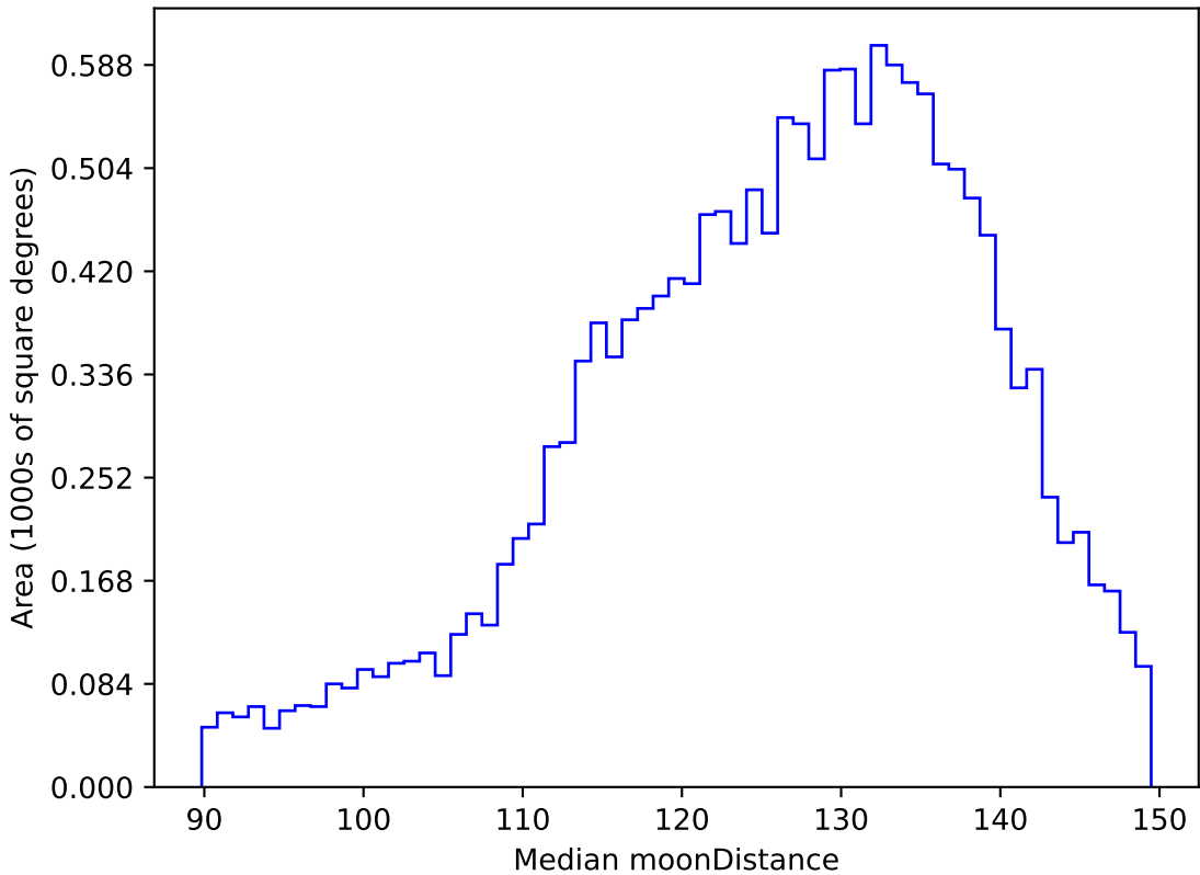
scp_reweight_v3.3_10yrs WFD u band: Median moonDistance
