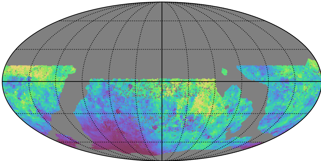
scp_reweight_v3.3_10yrs WFD r band: Median moonDistance
