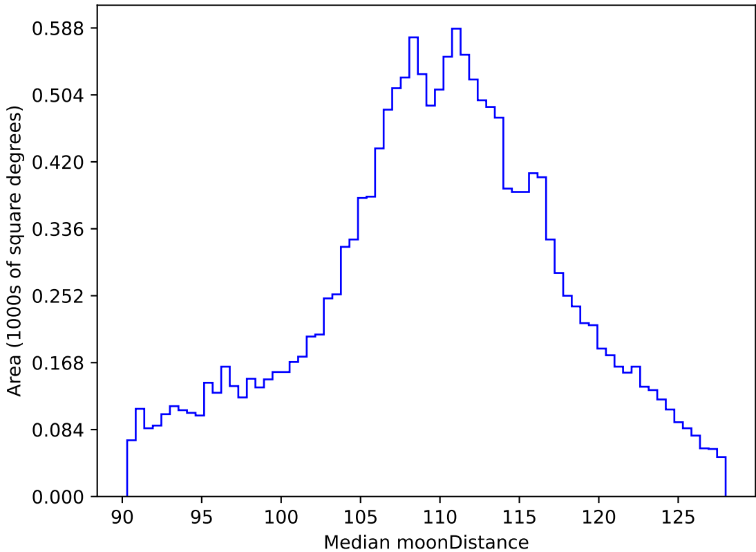
scp_reweight_v3.3_10yrs WFD r band: Median moonDistance
