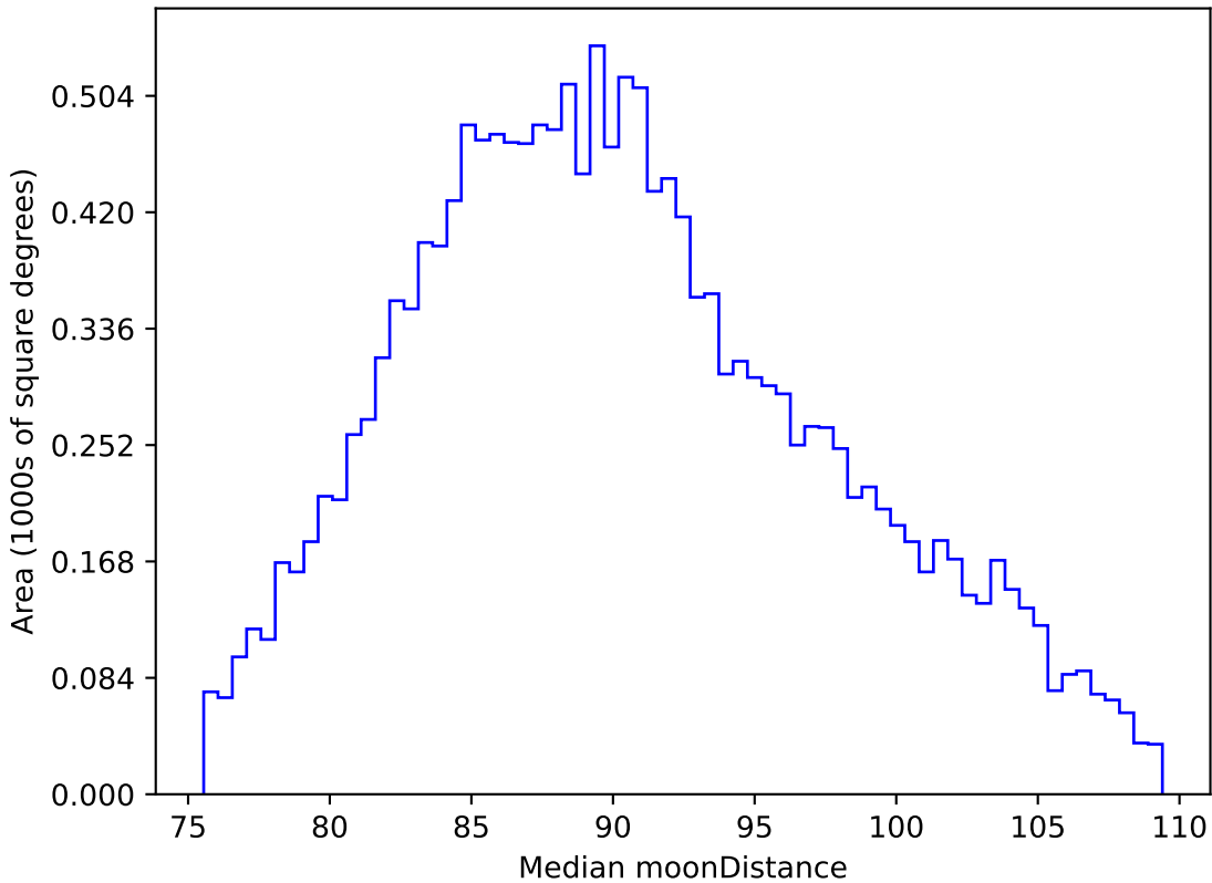
scp_reweight_v3.3_10yrs WFD i band: Median moonDistance
