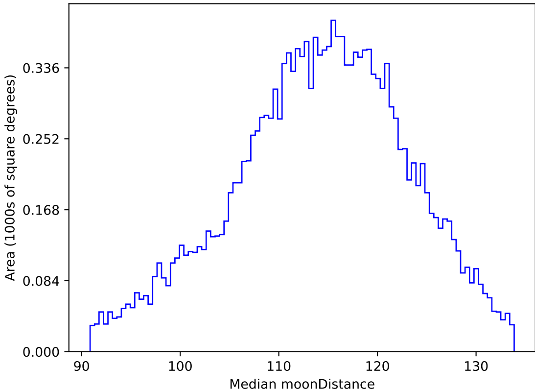
scp_reweight_v3.3_10yrs WFD g band: Median moonDistance
