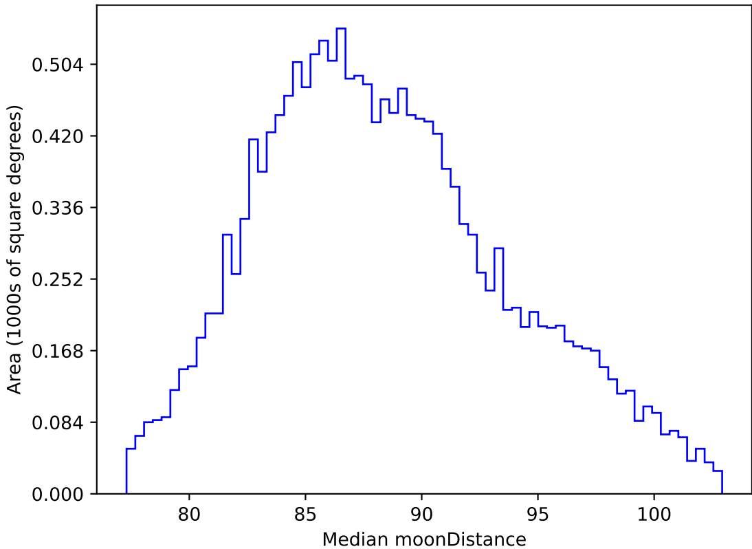
scp_reweight_v3.3_10yrs WFD all bands: Median moonDistance
