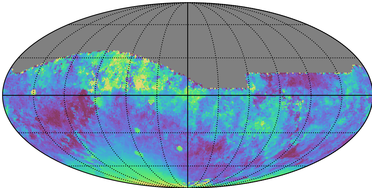
scp_reweight_v3.3_10yrs All sky z band: Median moonDistance
