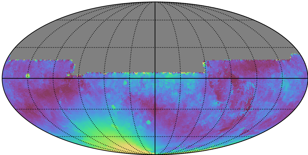
scp_reweight_v3.3_10yrs All sky y band: Median moonDistance
