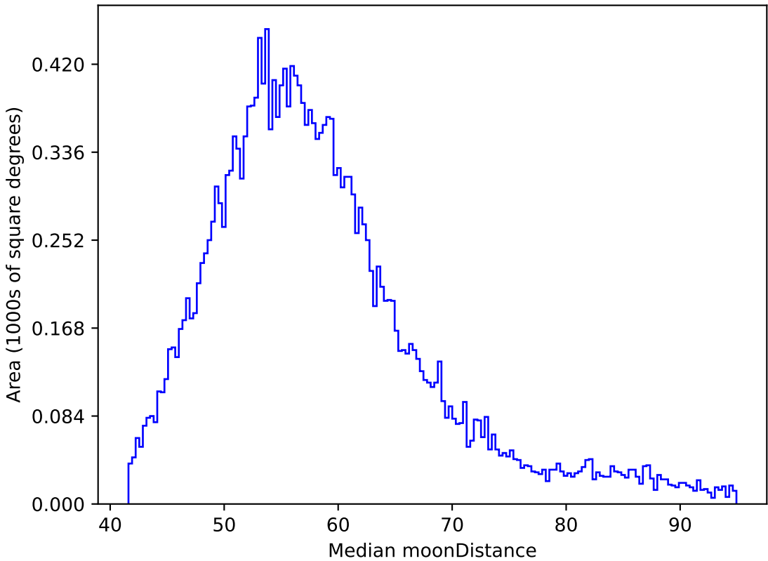
scp_reweight_v3.3_10yrs All sky y band: Median moonDistance
