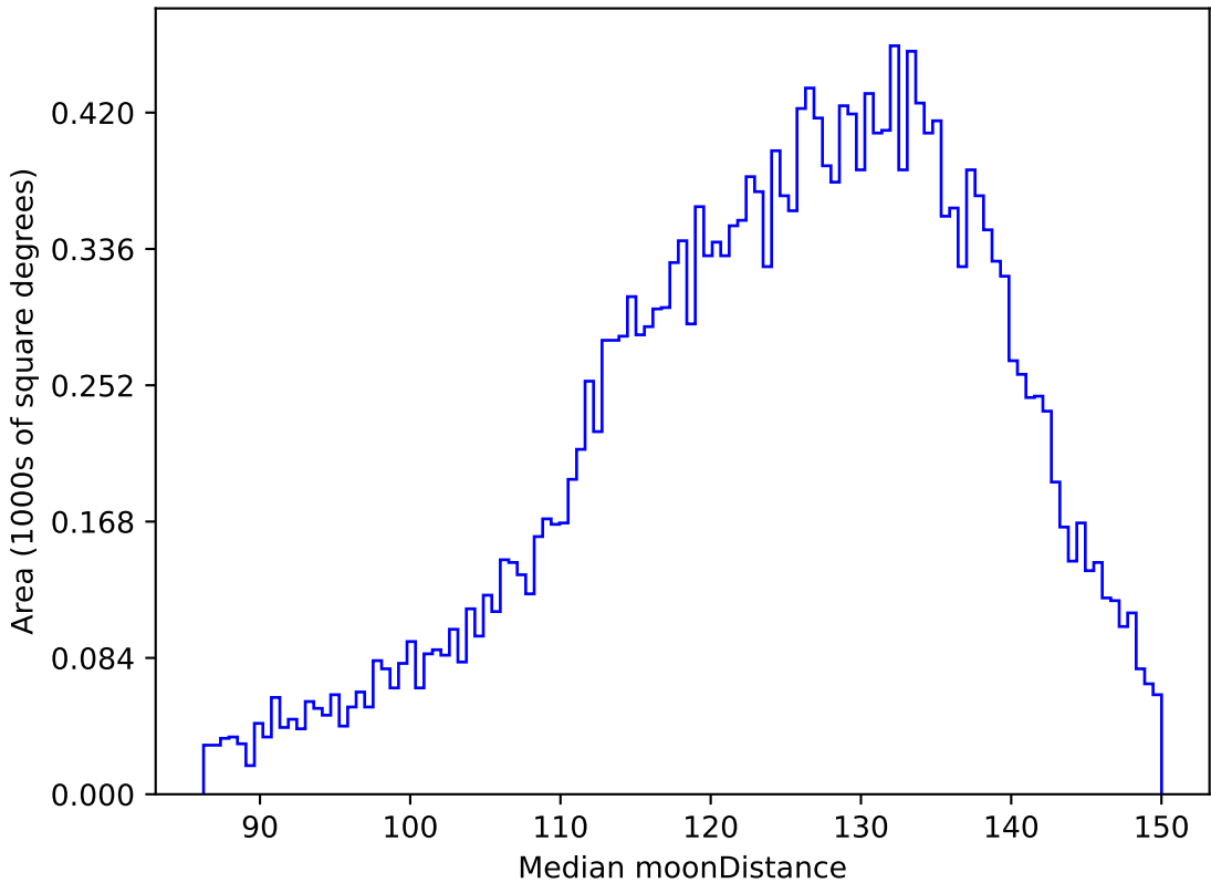
scp_reweight_v3.3_10yrs All sky u band: Median moonDistance
