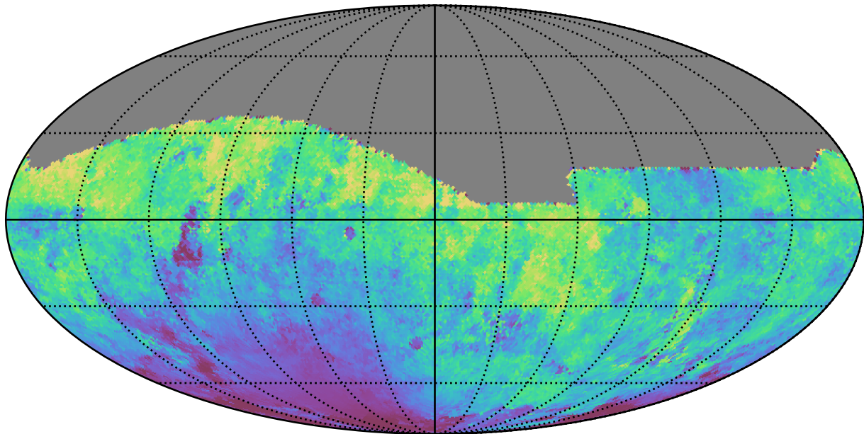
scp_reweight_v3.3_10yrs All sky r band: Median moonDistance
