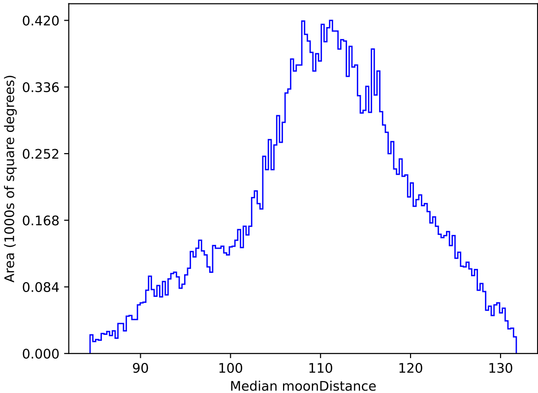
scp_reweight_v3.3_10yrs All sky r band: Median moonDistance
