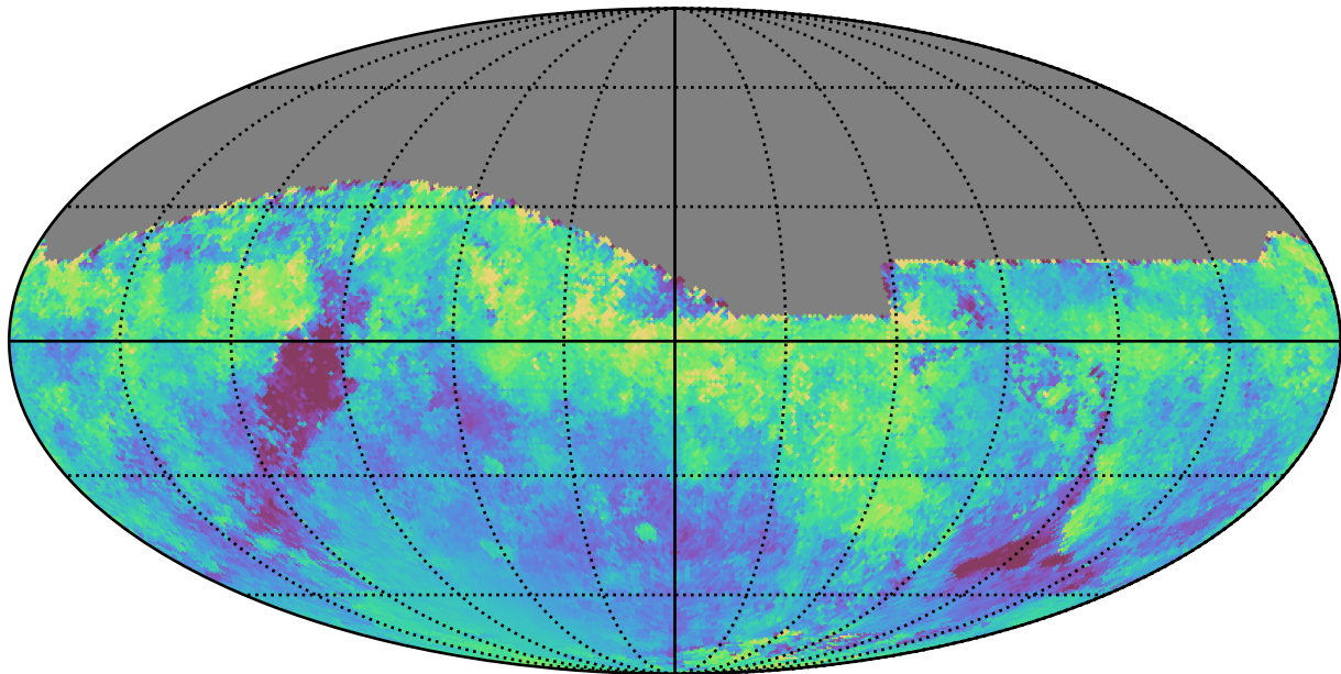
scp_reweight_v3.3_10yrs All sky i band: Median moonDistance
