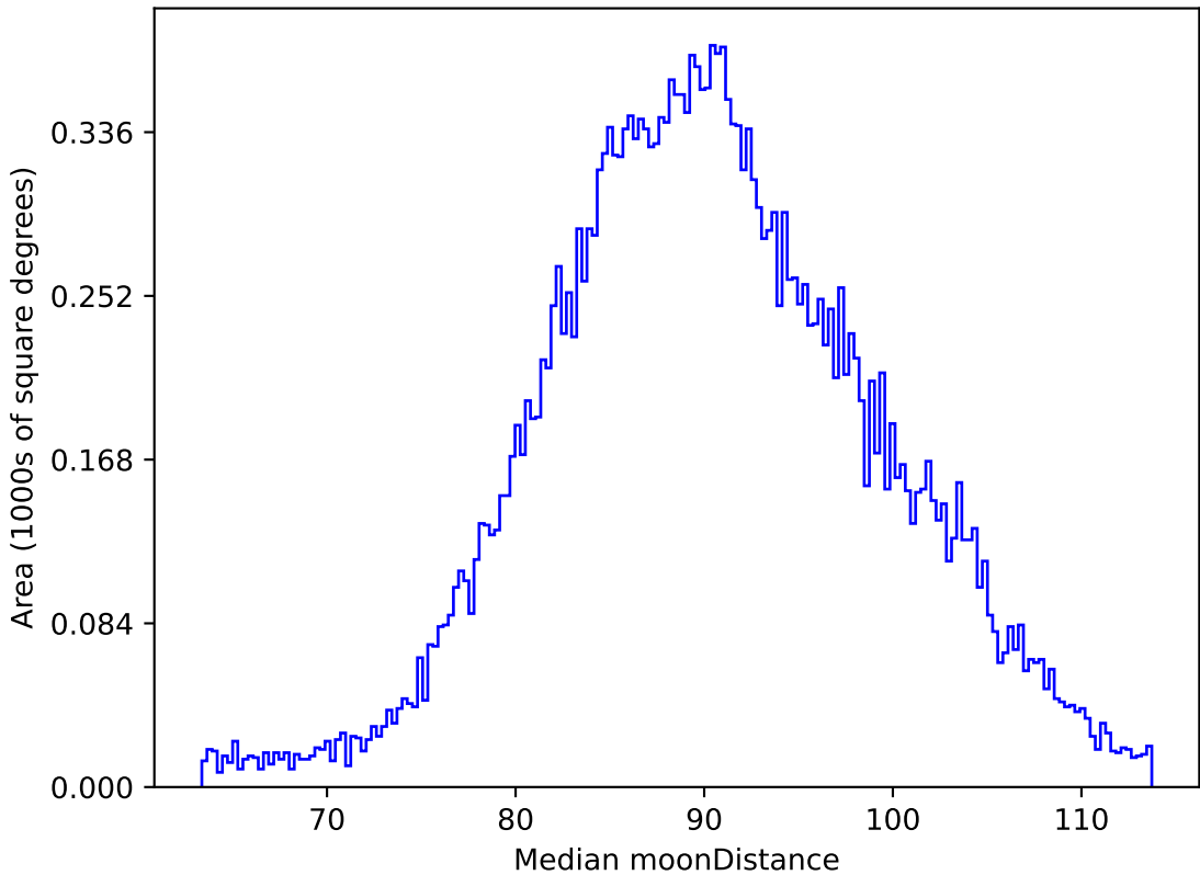
scp_reweight_v3.3_10yrs All sky i band: Median moonDistance
