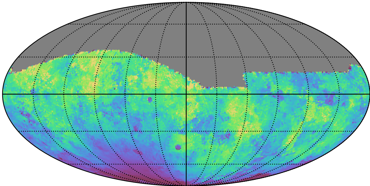
scp_reweight_v3.3_10yrs All sky g band: Median moonDistance
