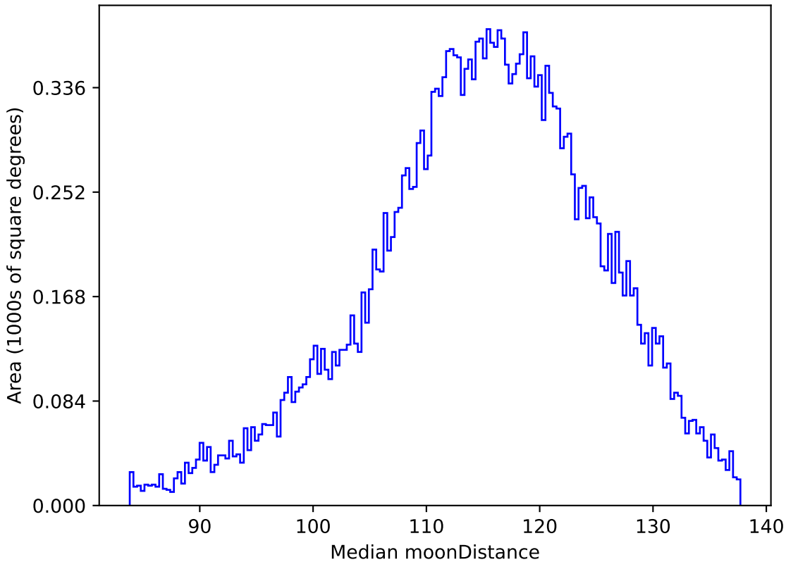
scp_reweight_v3.3_10yrs All sky g band: Median moonDistance
