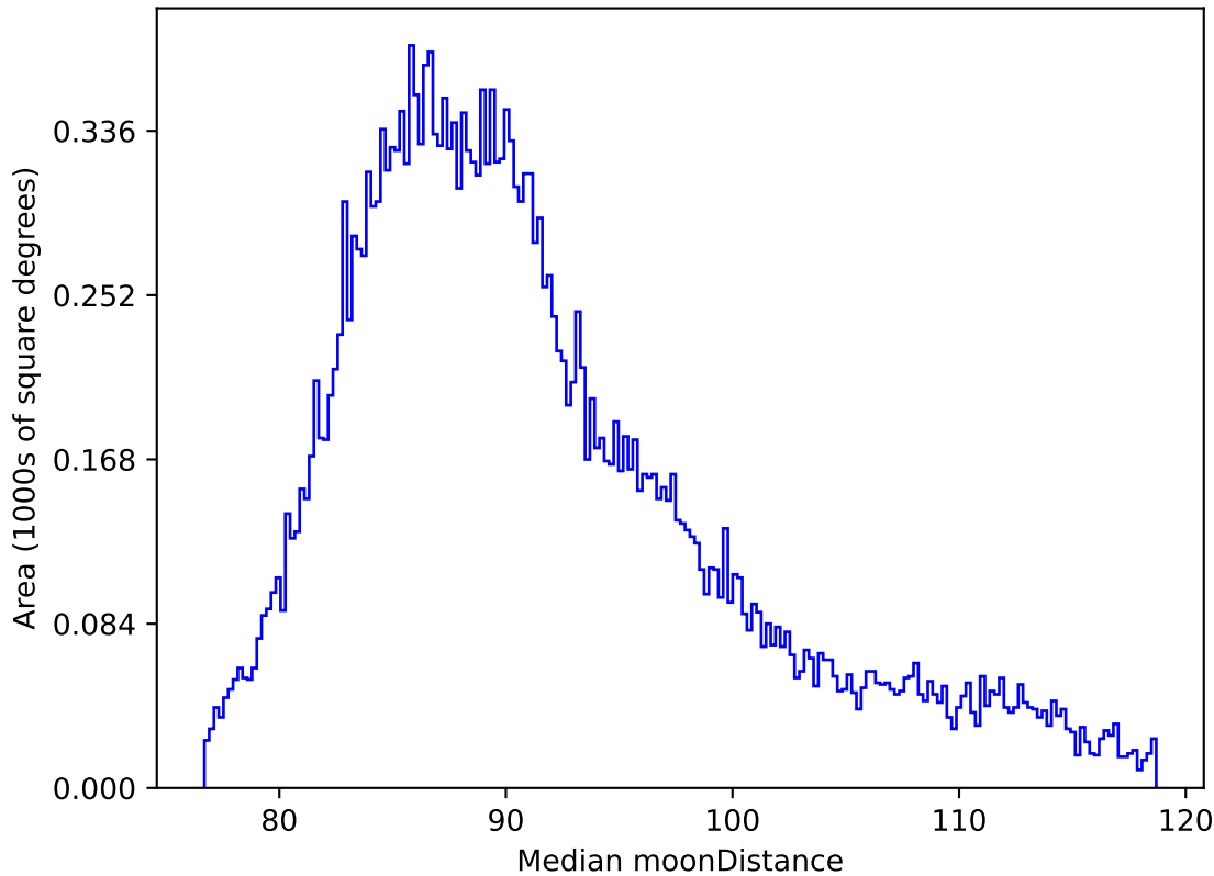
scp_reweight_v3.3_10yrs All sky all bands: Median moonDistance
