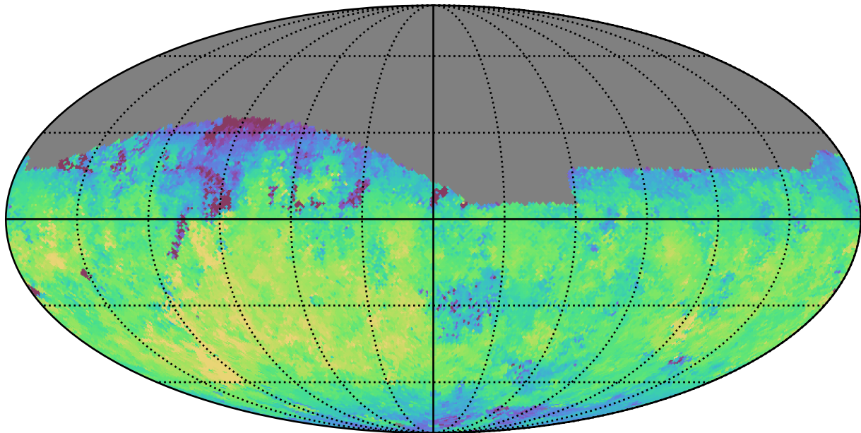
scp_reweight_v3.3_10yrs Yr 1 z band: Median fiveSigmaDepth
