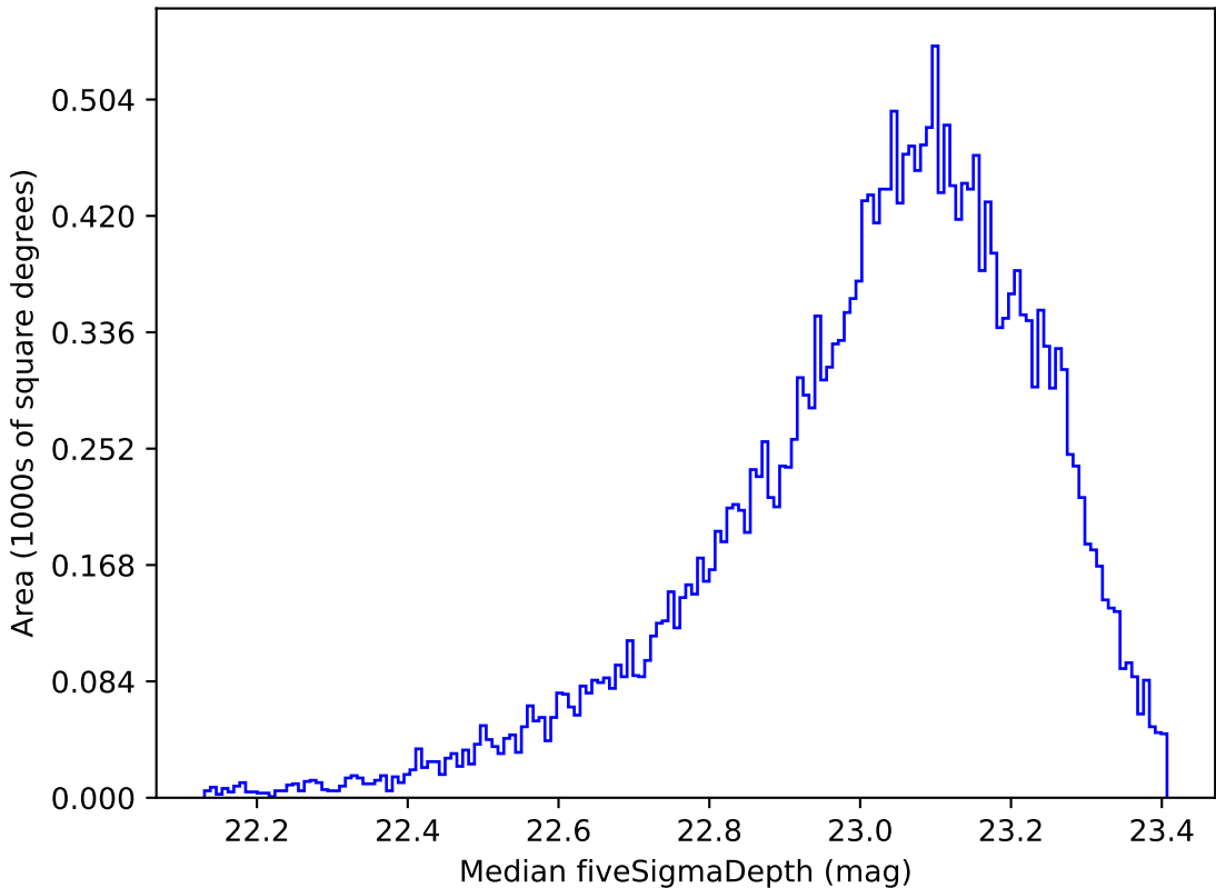
scp_reweight_v3.3_10yrs Yr 1 z band: Median fiveSigmaDepth
