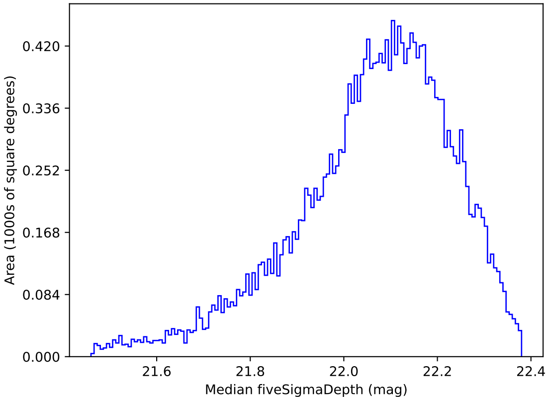
scp_reweight_v3.3_10yrs Yr 1 y band: Median fiveSigmaDepth
