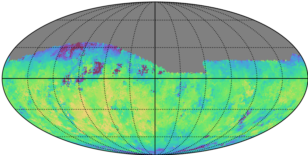
scp_reweight_v3.3_10yrs Yr 1 r band: Median fiveSigmaDepth
