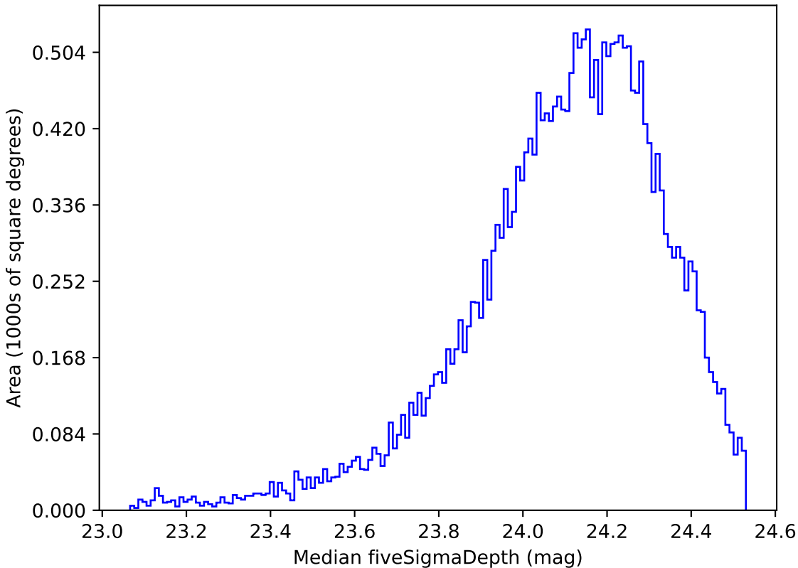
scp_reweight_v3.3_10yrs Yr 1 r band: Median fiveSigmaDepth
