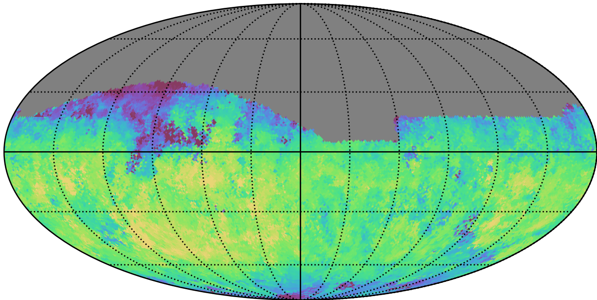
scp_reweight_v3.3_10yrs Yr 1 i band: Median fiveSigmaDepth
