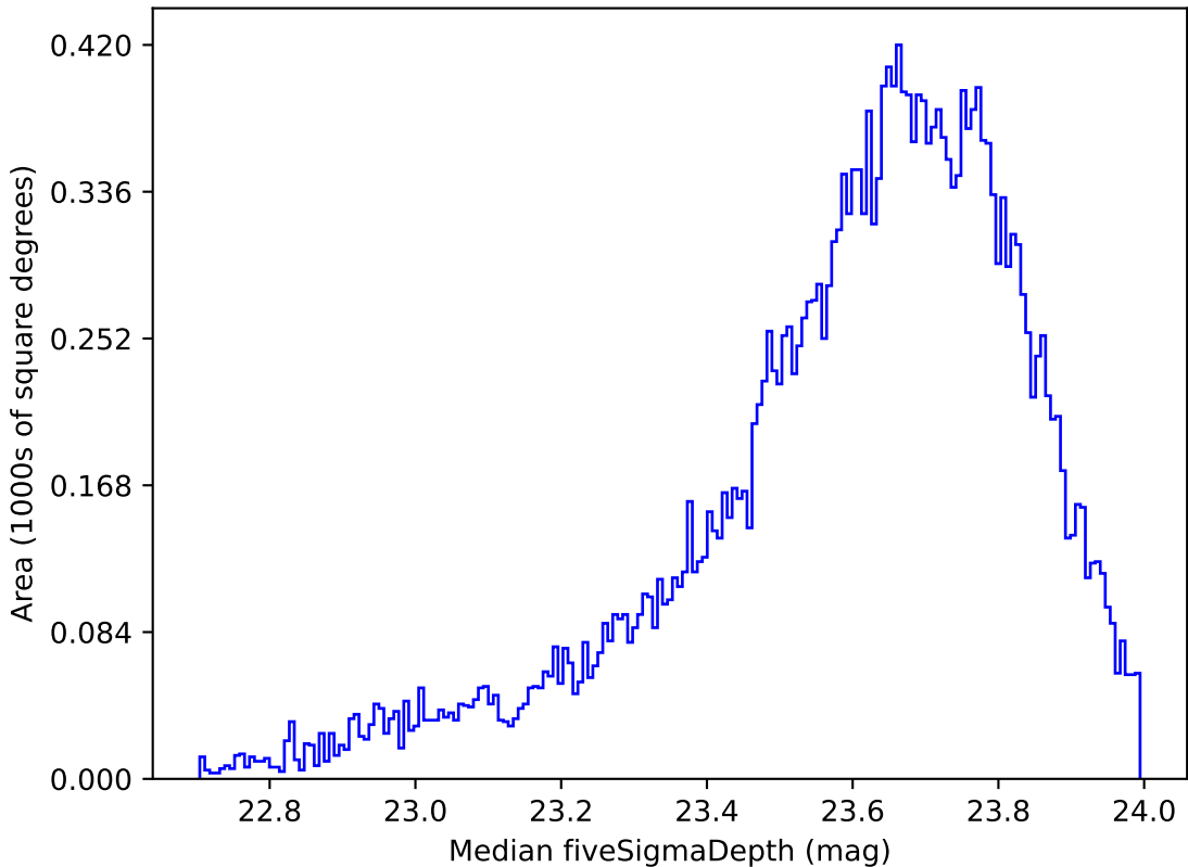
scp_reweight_v3.3_10yrs Yr 1 i band: Median fiveSigmaDepth
