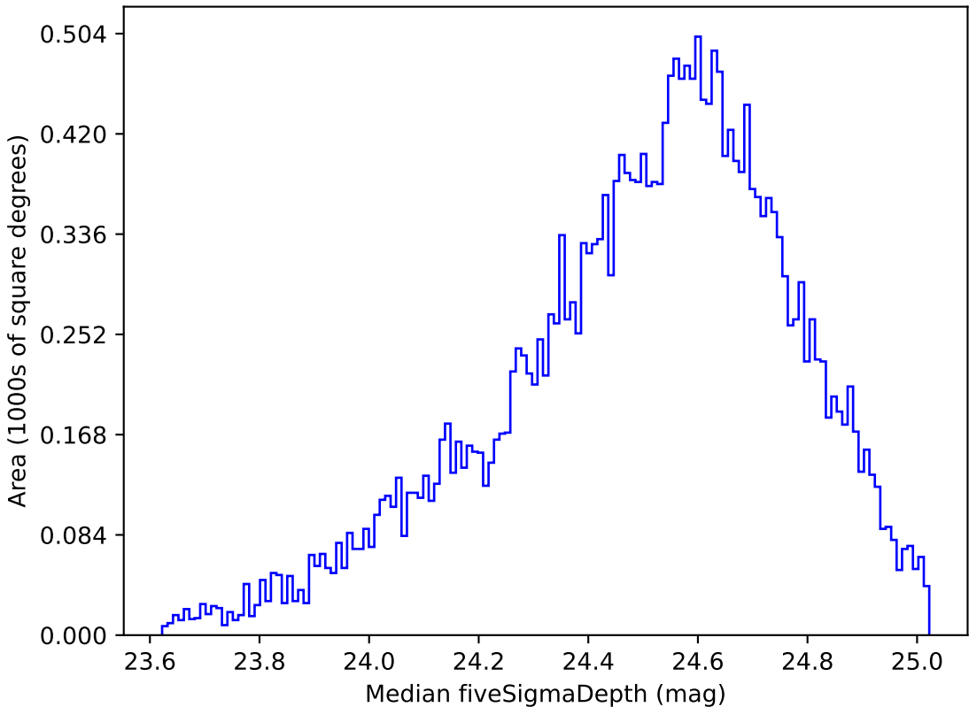
scp_reweight_v3.3_10yrs Yr 1 g band: Median fiveSigmaDepth
