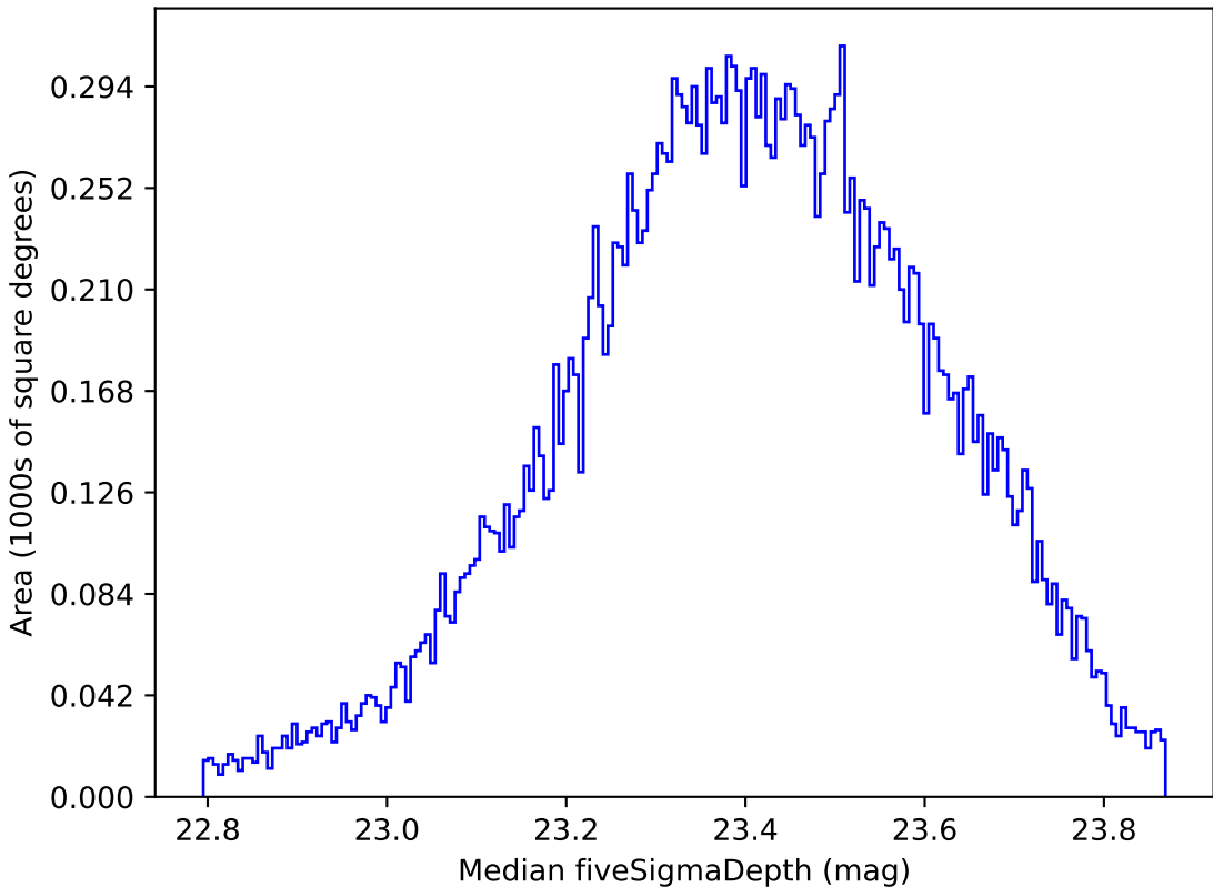
scp_reweight_v3.3_10yrs Yr 1 all bands: Median fiveSigmaDepth
