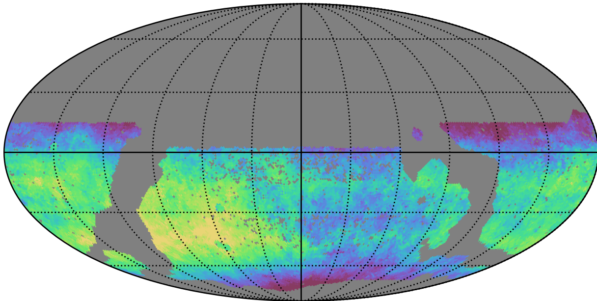
scp_reweight_v3.3_10yrs WFD z band: Median fiveSigmaDepth
