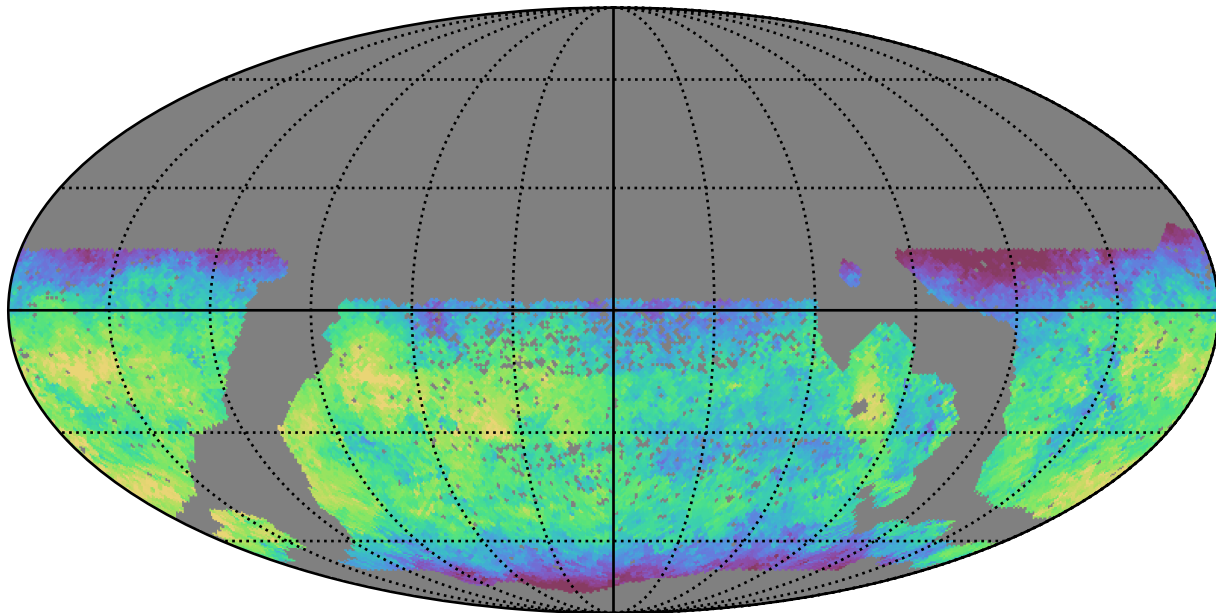
scp_reweight_v3.3_10yrs WFD u band: Median fiveSigmaDepth
