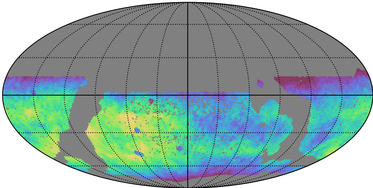
scp_reweight_v3.3_10yrs WFD r band: Median fiveSigmaDepth
