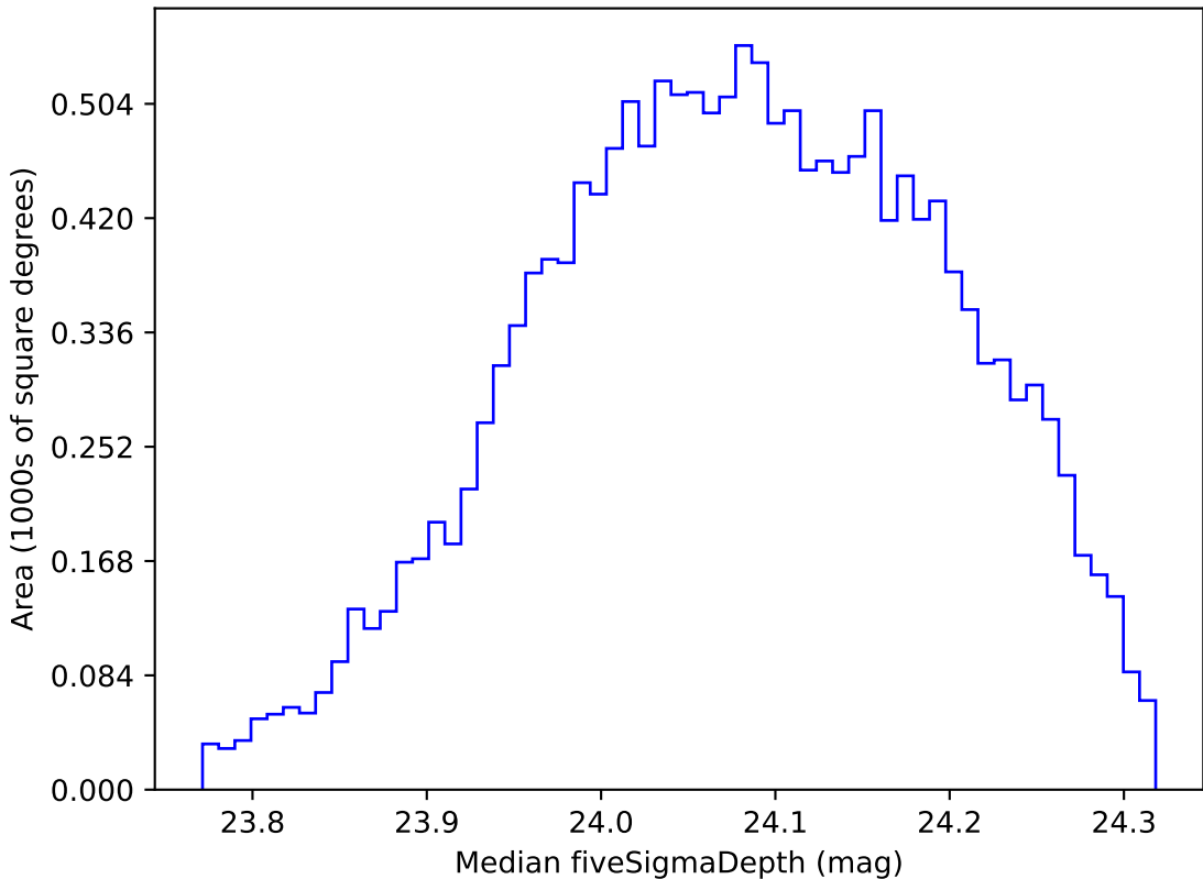
scp_reweight_v3.3_10yrs WFD r band: Median fiveSigmaDepth
