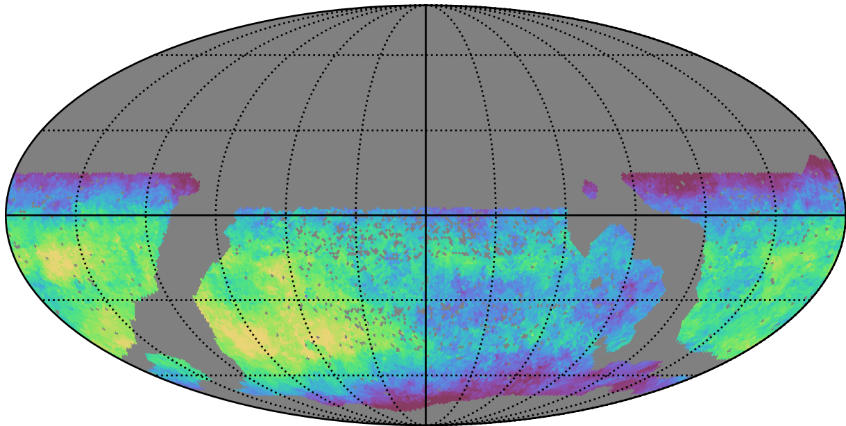
scp_reweight_v3.3_10yrs WFD i band: Median fiveSigmaDepth
