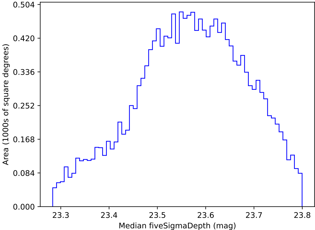
scp_reweight_v3.3_10yrs WFD i band: Median fiveSigmaDepth
