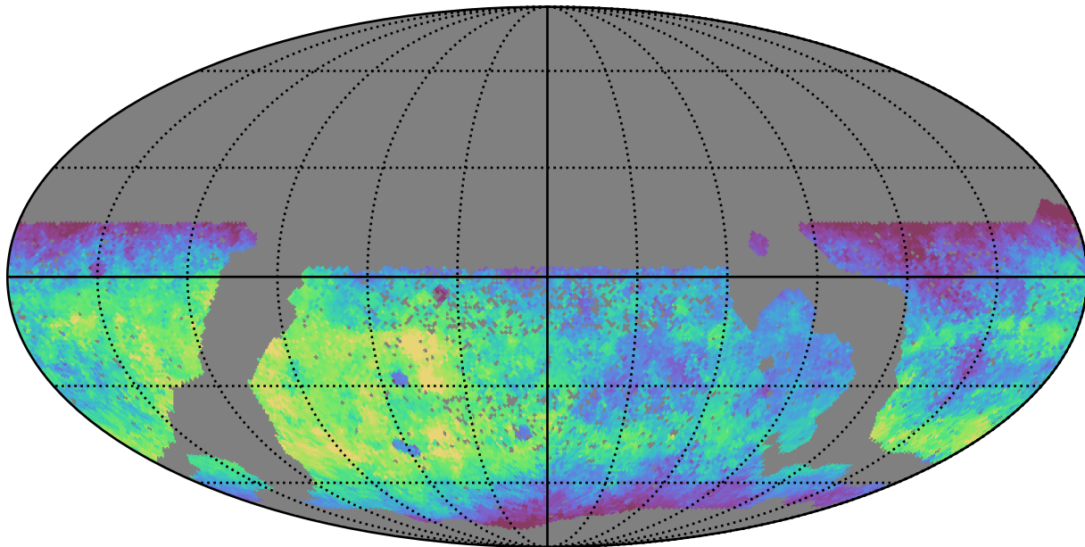
scp_reweight_v3.3_10yrs WFD g band: Median fiveSigmaDepth
