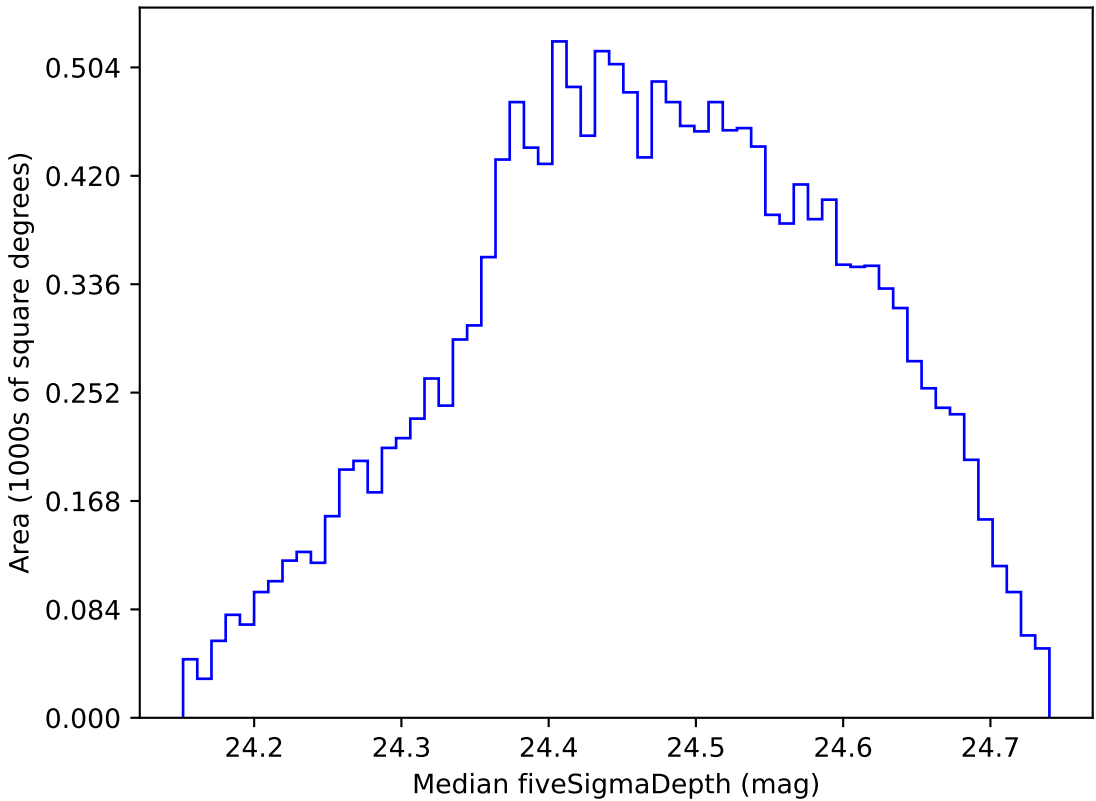
scp_reweight_v3.3_10yrs WFD g band: Median fiveSigmaDepth
