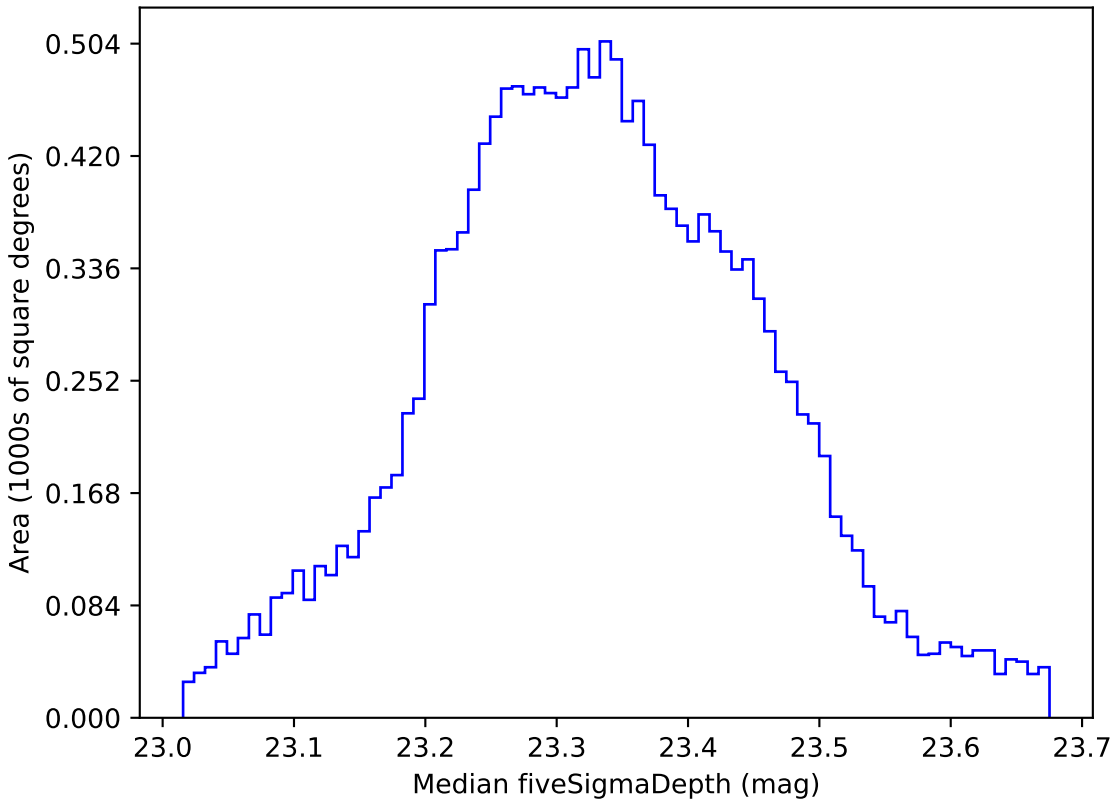
scp_reweight_v3.3_10yrs WFD all bands: Median fiveSigmaDepth
