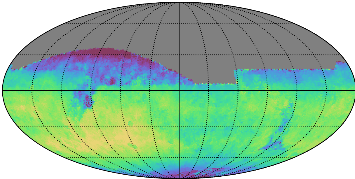
scp_reweight_v3.3_10yrs All sky z band: Median fiveSigmaDepth
