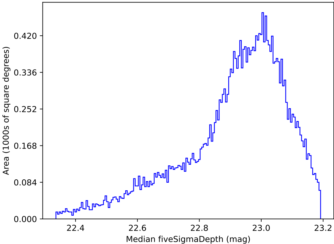
scp_reweight_v3.3_10yrs All sky z band: Median fiveSigmaDepth
