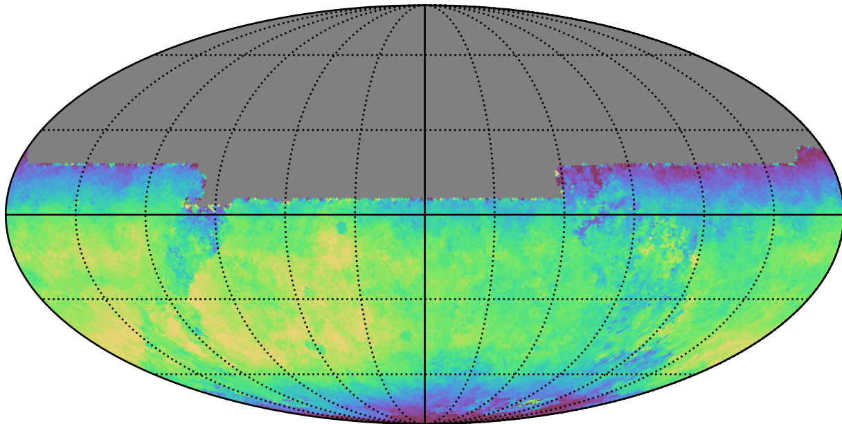
scp_reweight_v3.3_10yrs All sky y band: Median fiveSigmaDepth
