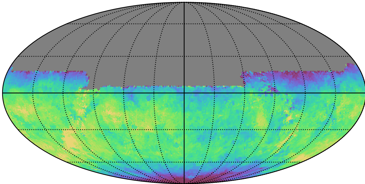
scp_reweight_v3.3_10yrs All sky u band: Median fiveSigmaDepth
