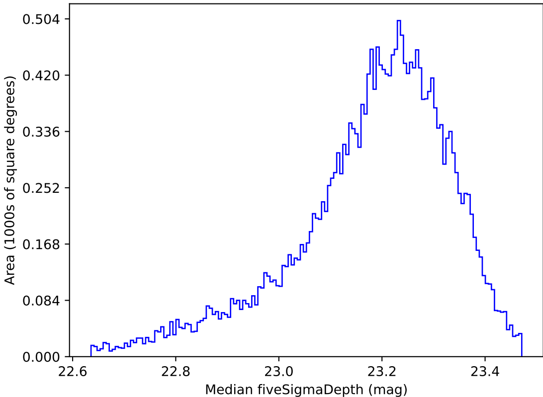
scp_reweight_v3.3_10yrs All sky u band: Median fiveSigmaDepth
