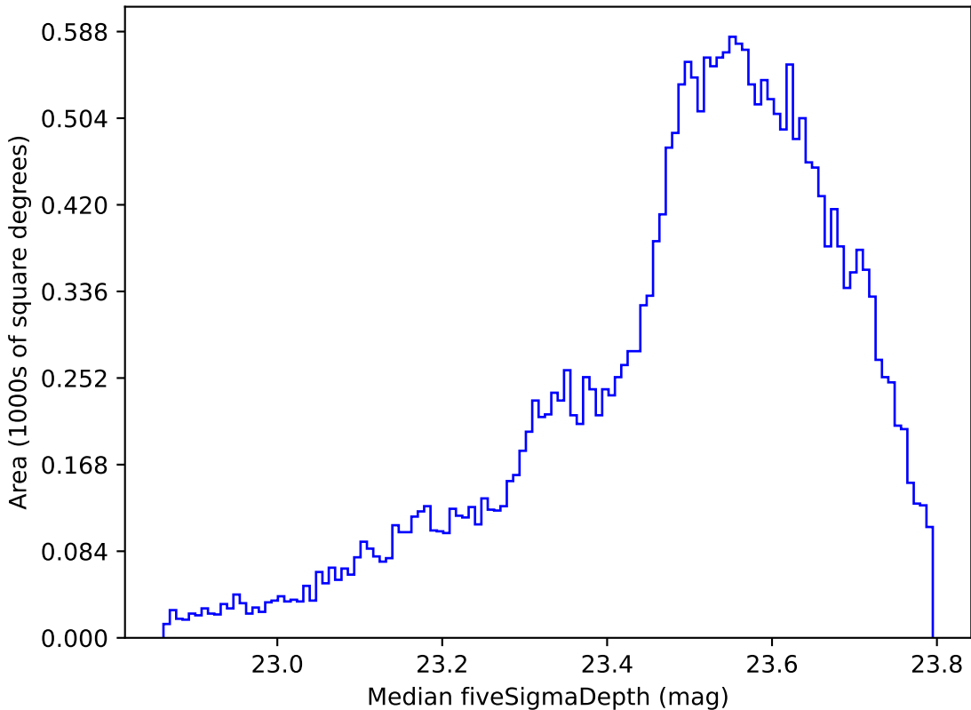
scp_reweight_v3.3_10yrs All sky i band: Median fiveSigmaDepth
