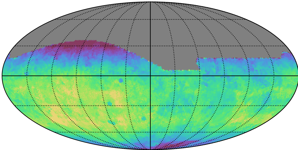
scp_reweight_v3.3_10yrs All sky g band: Median fiveSigmaDepth
