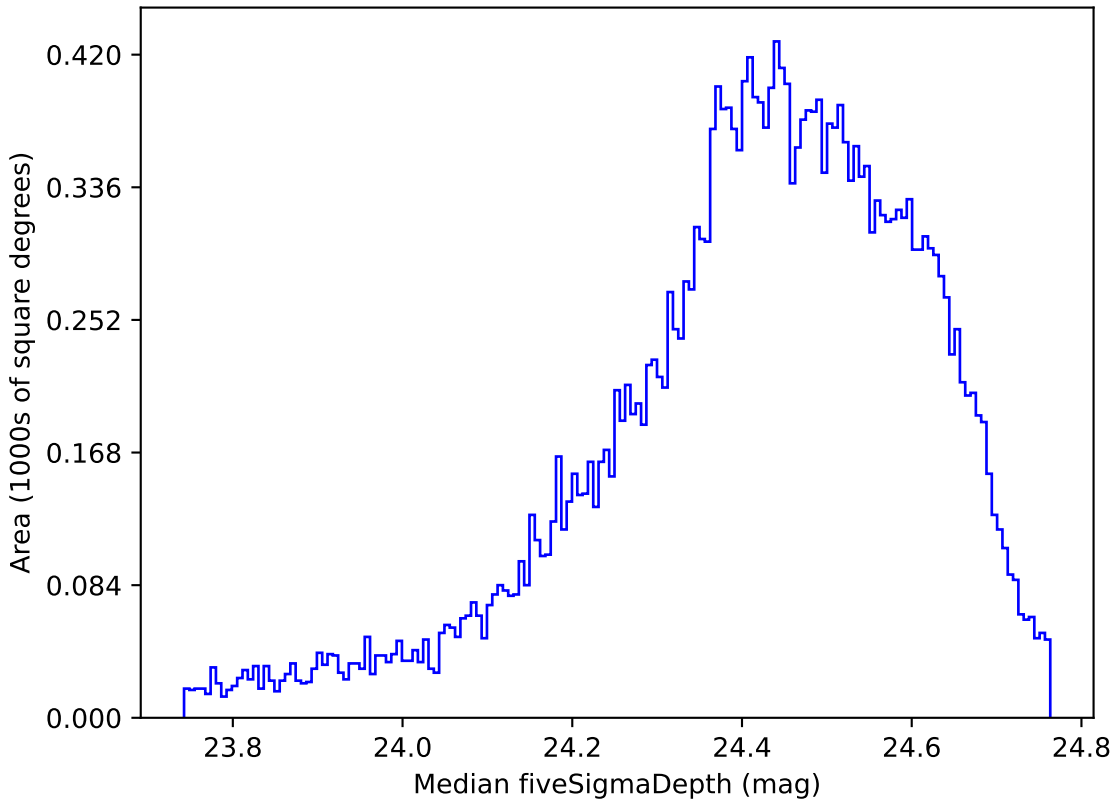
scp_reweight_v3.3_10yrs All sky g band: Median fiveSigmaDepth
