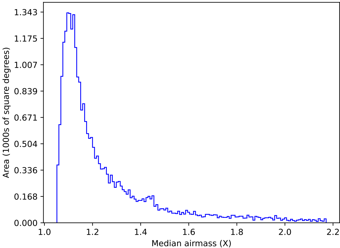
scp_reweight_v3.3_10yrs Yr 1 z band: Median airmass
